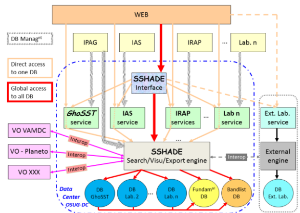
Figure 2: Schematic structure of SSHADE infrastructure
